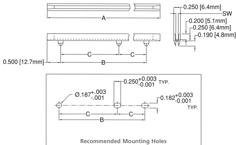
Recommended Mounting Holes
